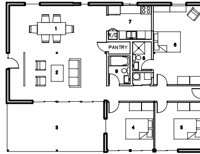
2 ALTERNATE FLOOR PLAN NTS
