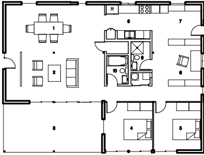
1 ALTERNATE FLOOR PLAN NTS
