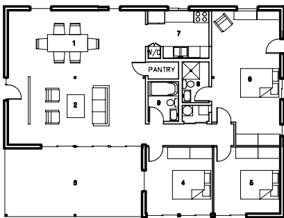
4 ALTERNATE FLOOR PLAN NTS
