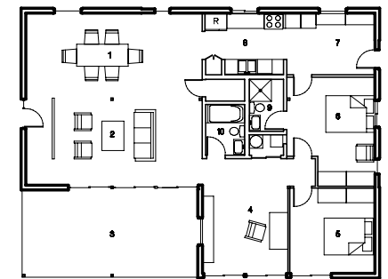
6 ALTERNATE FLOOR PLAN NTS
