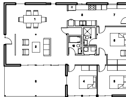
5 ALTERNATE FLOOR PLAN NTS
